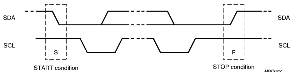
Fig.8 Start and stop conditions.
