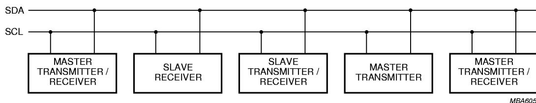
Fig.9 System configuration.
