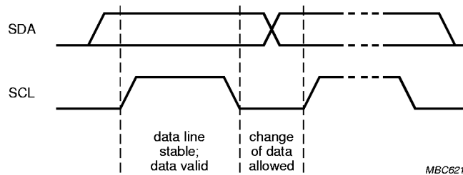
Fig.7 Bit transfer.
